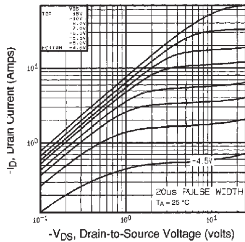
Fig. 1 - Typical Output Characteristics, T_A = 25\text{ °C}
